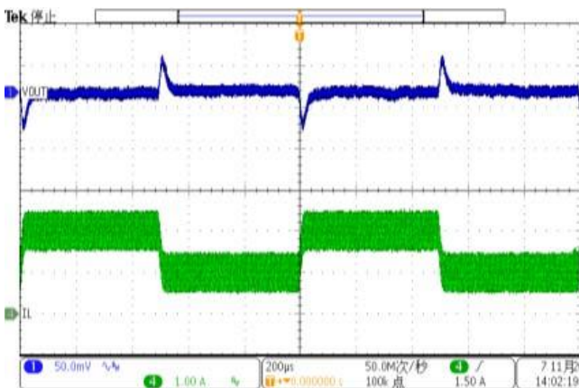
Loop Response VIN = 12V, VOUT = 3.3V, IOU = 1A-2A
