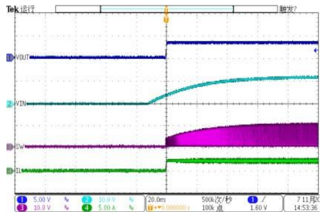
Power Up at Full Load VIN = 12V, VOUT = 3.3V, IOU = 2A
