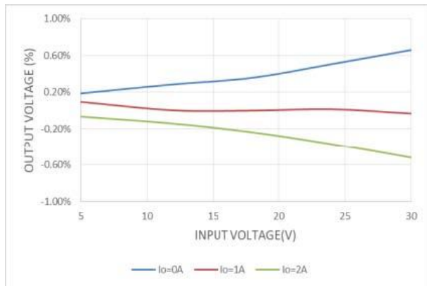
Line Regulation VOUT = 3.3V
