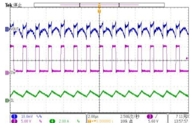
Output Ripple Voltage VIN = 12V, VOUT = 3.3V, IOU = 1A
