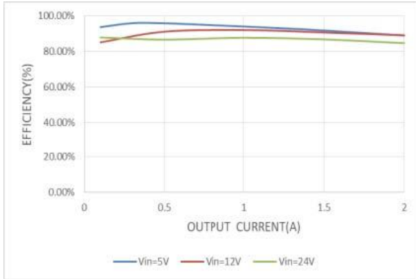
Efficiency vs Load Current VOUT = 3.3V
