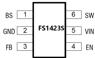
6-LEAD PLASTIC SOT-23
