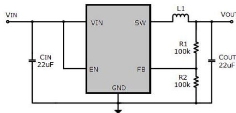
Figure 1. Basic Application Circuit
