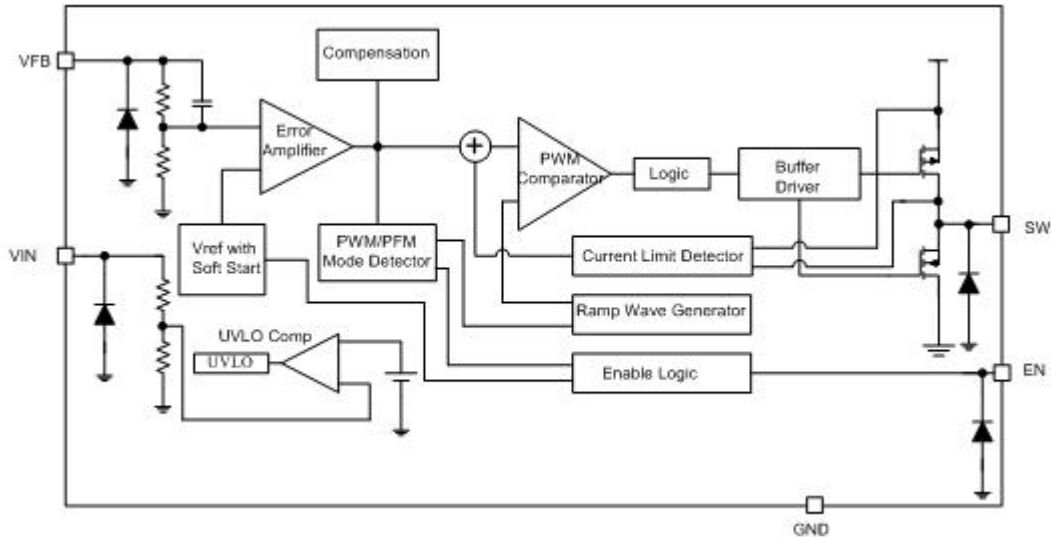
Figure 2. FS3430 Block Diagram
